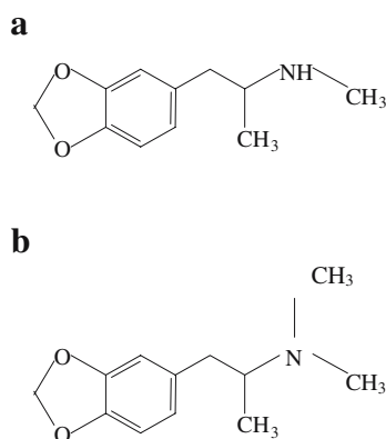
Fig. 1 Chemical structure of a 3,4-methylenedioxymethamphetamine (MDMA) and b 3,4-methylenedioxy- N,N -dimethylamphetamine (MDDM/MDDA)
